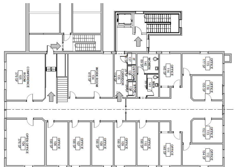
Third floor - Faculty offices and conference areas
